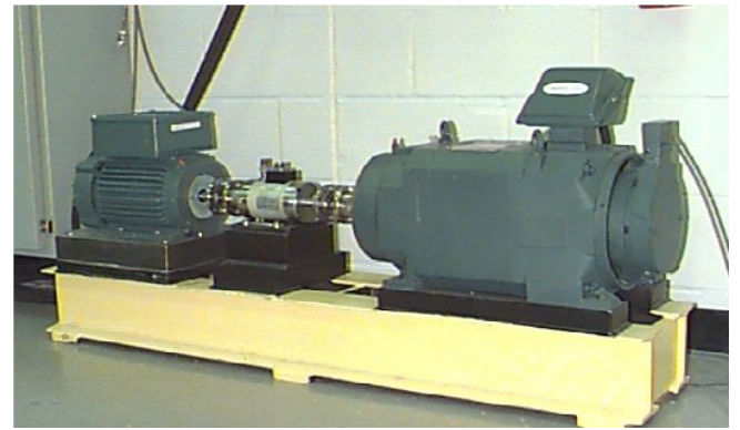
FIGURE 1. Test set up for CWRU bearing dataset [7]
