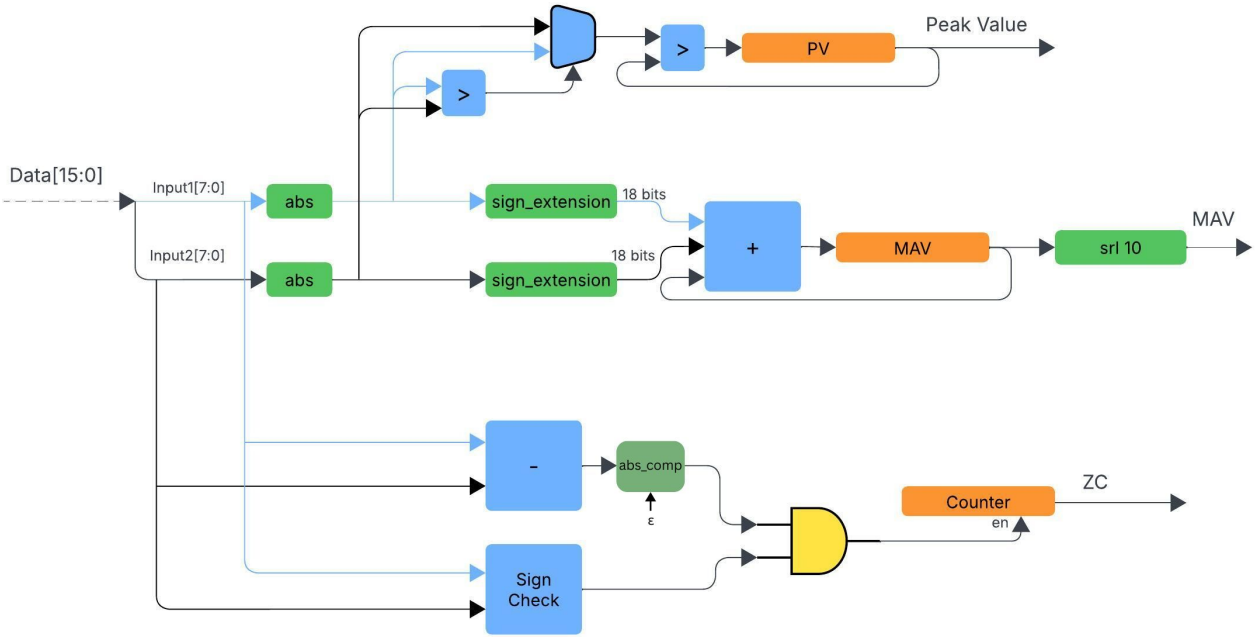
FIGURE 7. Datapath of the Feature Extraction Unit.
