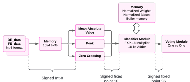
FIGURE 5. Single- and Multi-Variate architecture
