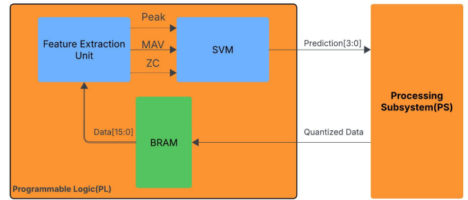
FIGURE 6. Overall FPGA accelerator architecture.
